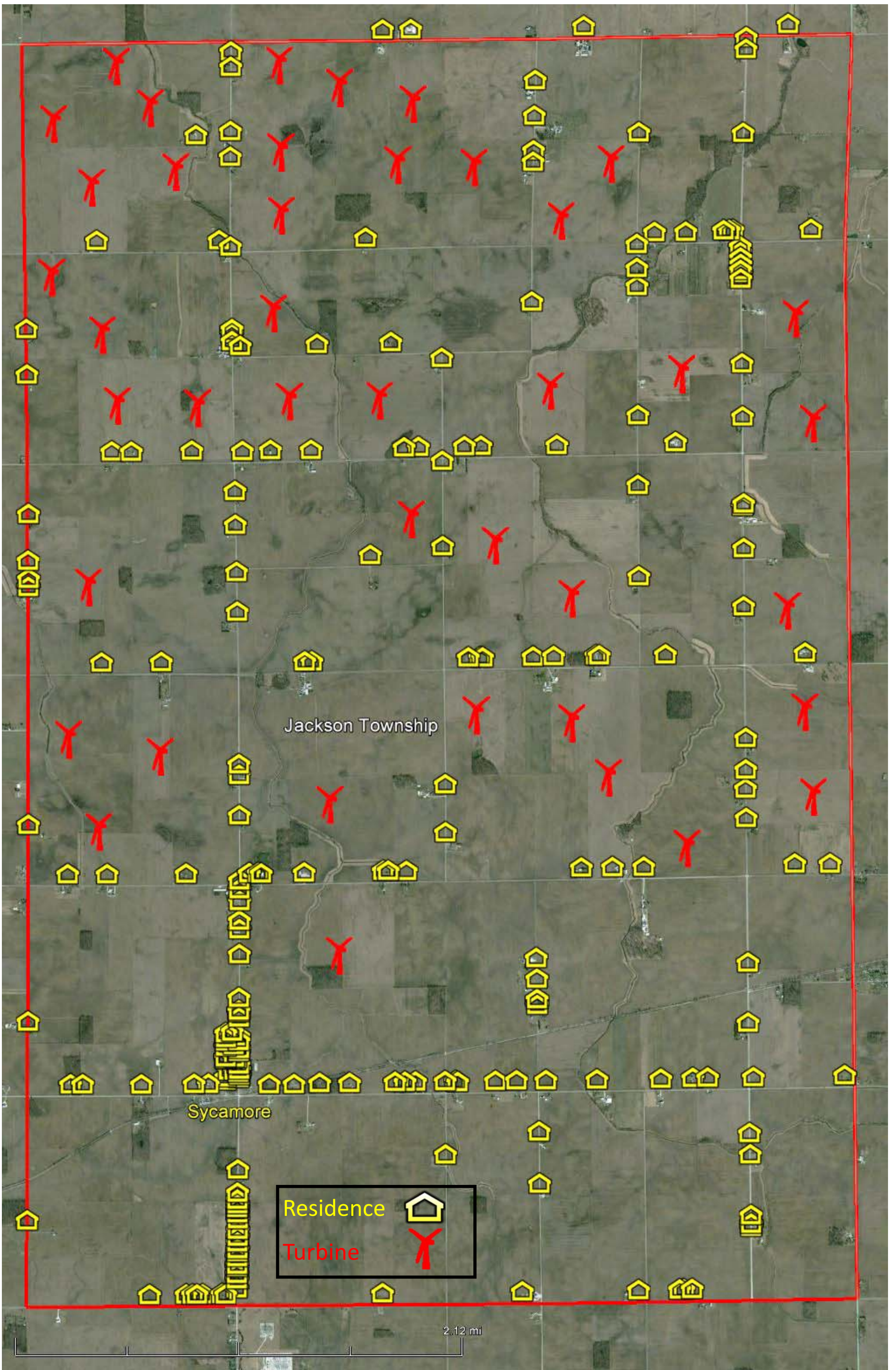
Map illustrating home density and proposed turbines in Howard County — Jackson Township—2010 Census—Population Density 25.4 per square mile
